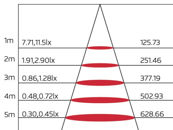
H(m) Eavg, Emax Beam Angle: 117.12 ° Diameter
