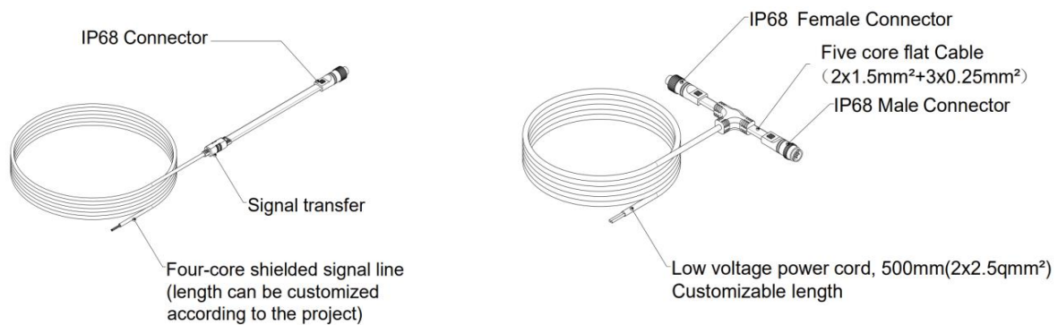
Power T Connector
